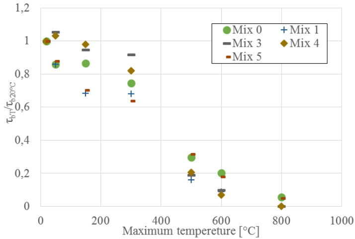
Figure 5: Test result on bond strength measured on ribbed reinforcement (every point gives the average of 3 measurements)
