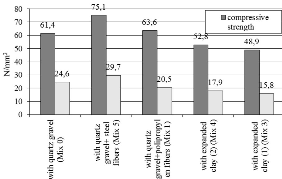
Figure 7: Concrete compressive strength and bond strength with various mixes at 20 °C
