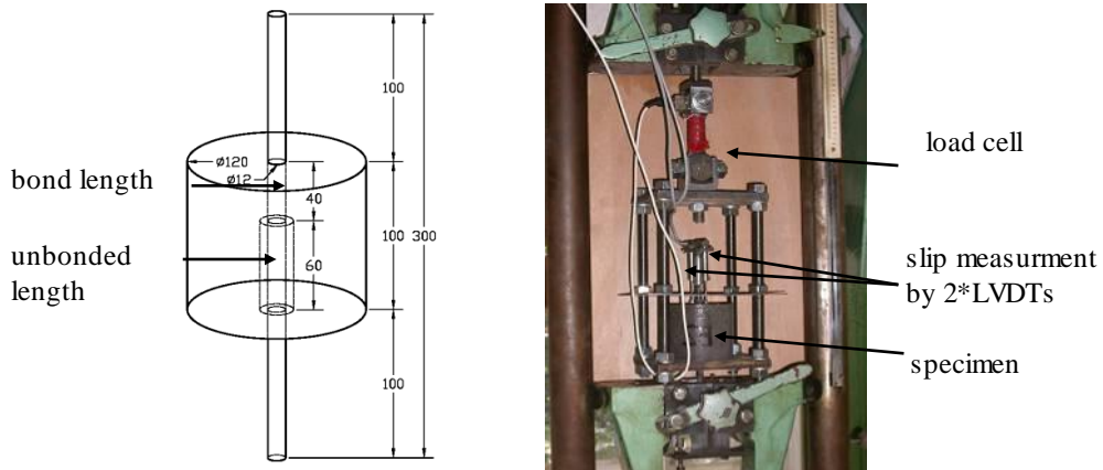
Figure 3: Pull-out tests a) Specimen b) test setup
