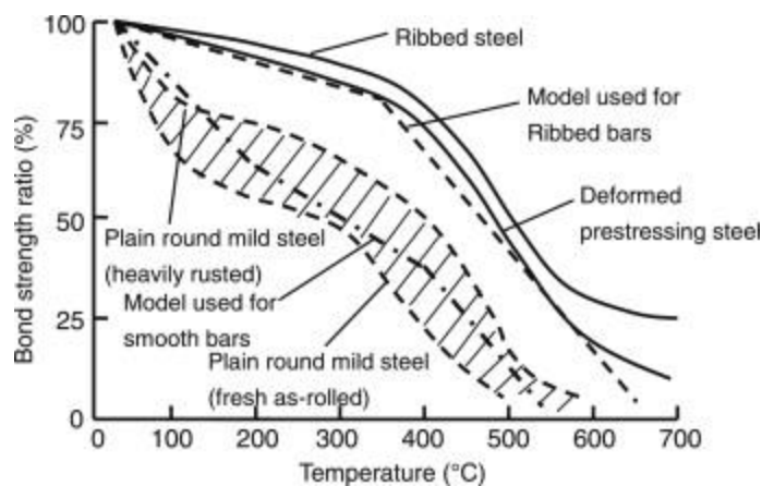
Figure 1: Degradation of bond strength between concrete and reinforcing steel [5]
