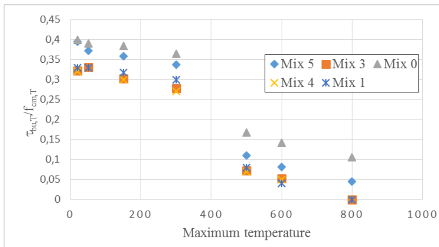
Figure 8: \tau_{bu,T}/f_{cm,T} as a function of maximum temperature in case of ribbed reinforcement
