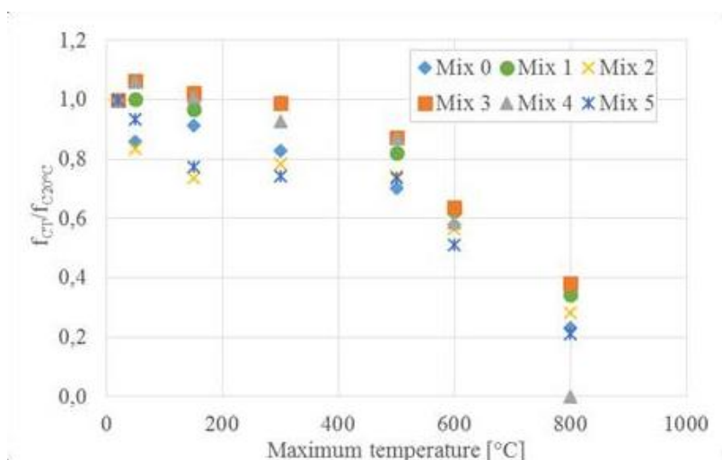
Figure 4: Relative residual compressive strength (every point gives the average of 3 measurements)
