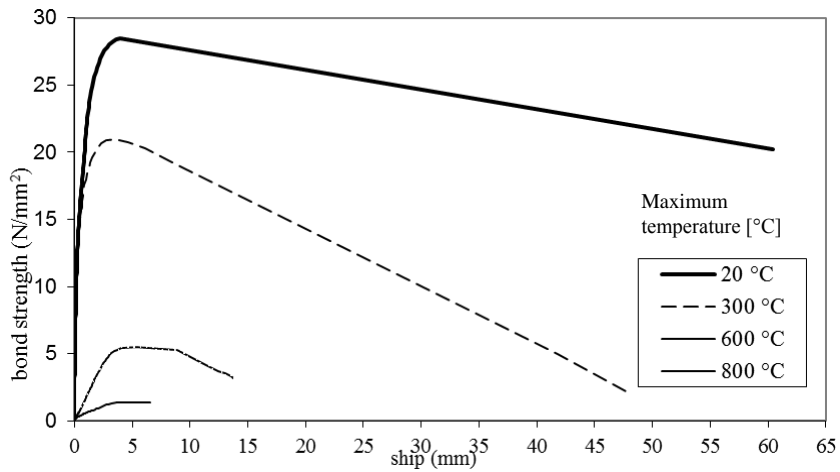
Figure 6: The \tau_b - slip diagram as a function of temperature (for Mix 0)
