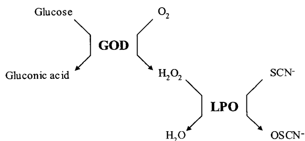
Figure 1. Overall reaction of hypothiocyanite formation by the lactoperoxidase system coupled with enzymatic generation of hydrogen peroxide
