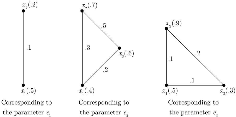
FIGURE 3. Spanning Fuzzy Soft subgraph.
