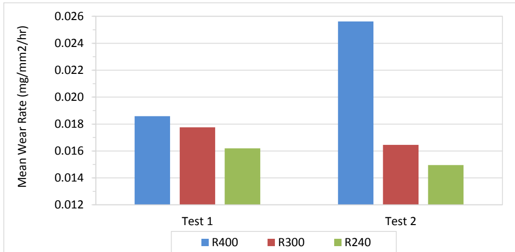
Figure 4. Wear Rates in the Small Mill
