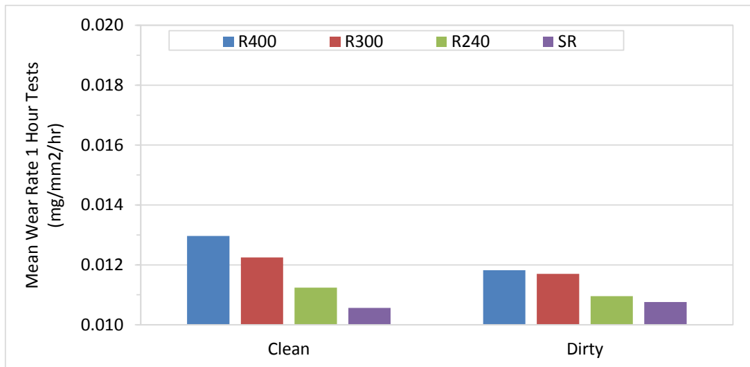
Figure 3. Effect of Surface Cleanliness on Mean Wear Rate, 3 Hour Tests
