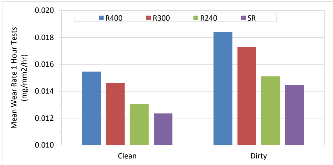
Figure 2. Effect of Surface Cleanliness on Mean Wear Rate, 1 Hour Tests
