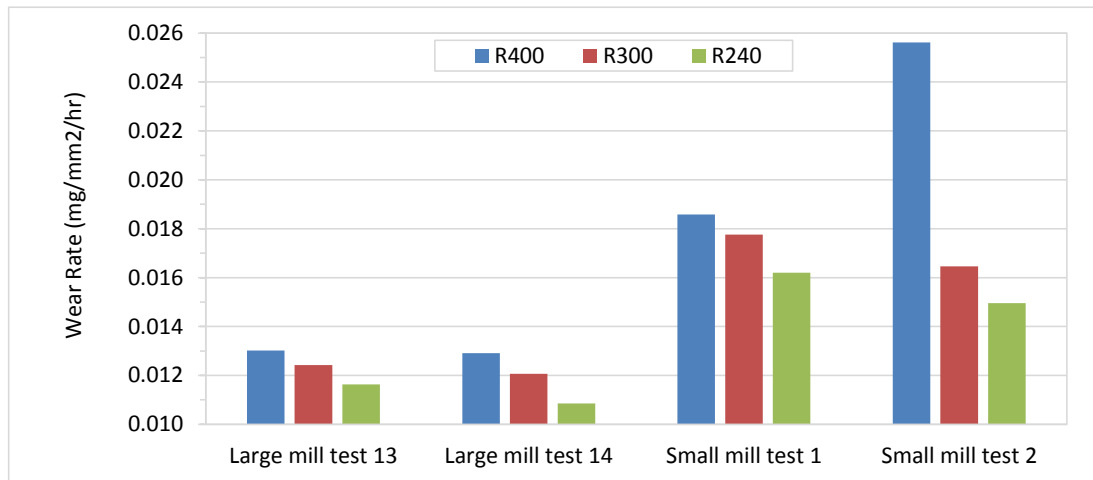
Figure 5. Comparison of Wear Rates from Large Mill and Small Mill Tests
