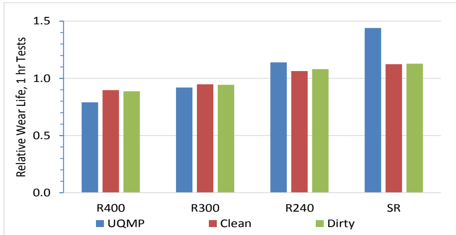
Figure 6. Relative Wear Life, One Hour Tests, Compared with UQMP Results
