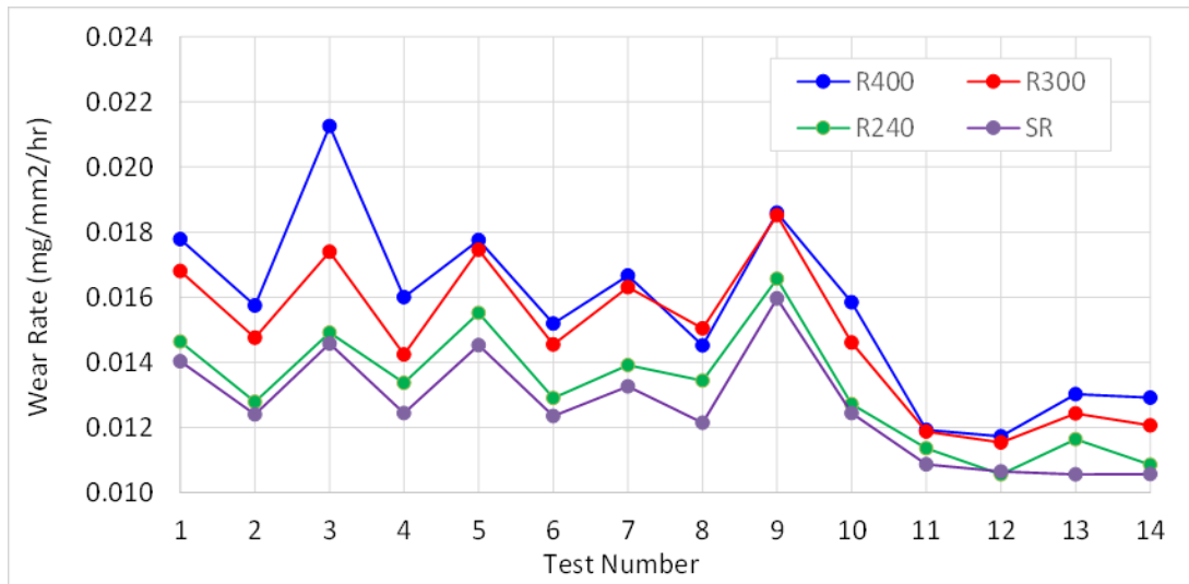
Figure 1. Wear Rates of Four Grades of Grinding Media in Successive Tests
