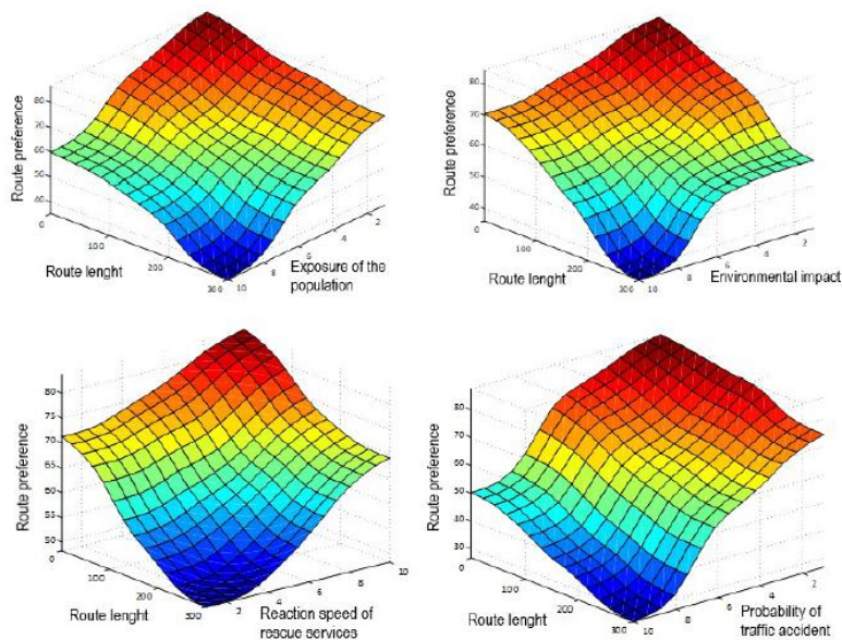
Figure 5. Interdependence of the solution and two input variables by the PROD-SUM method
