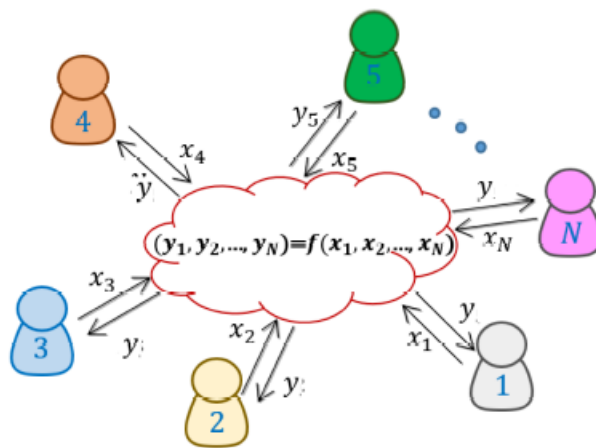
Figure 5 – Graphical presentation of the secure multiparty protocol
