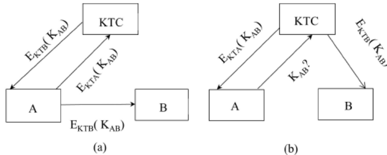
Figure 3 – Models of the Key translation center functioning
