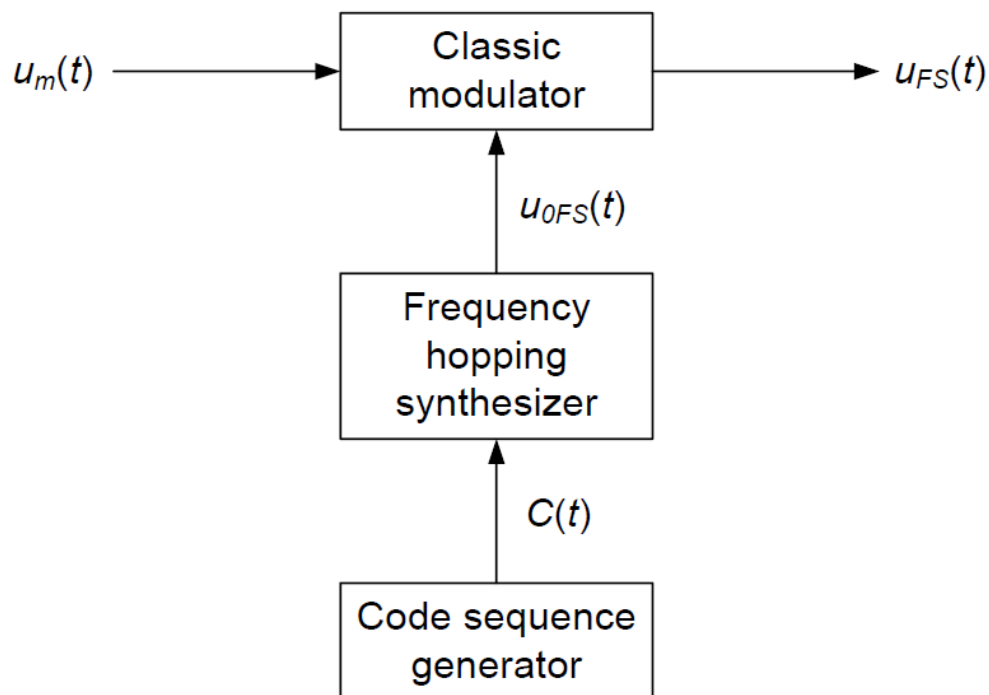
Figure 1 – FH-SS signal modulator
