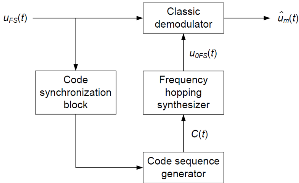
Figure 2 – FH-SS signal demodulator
