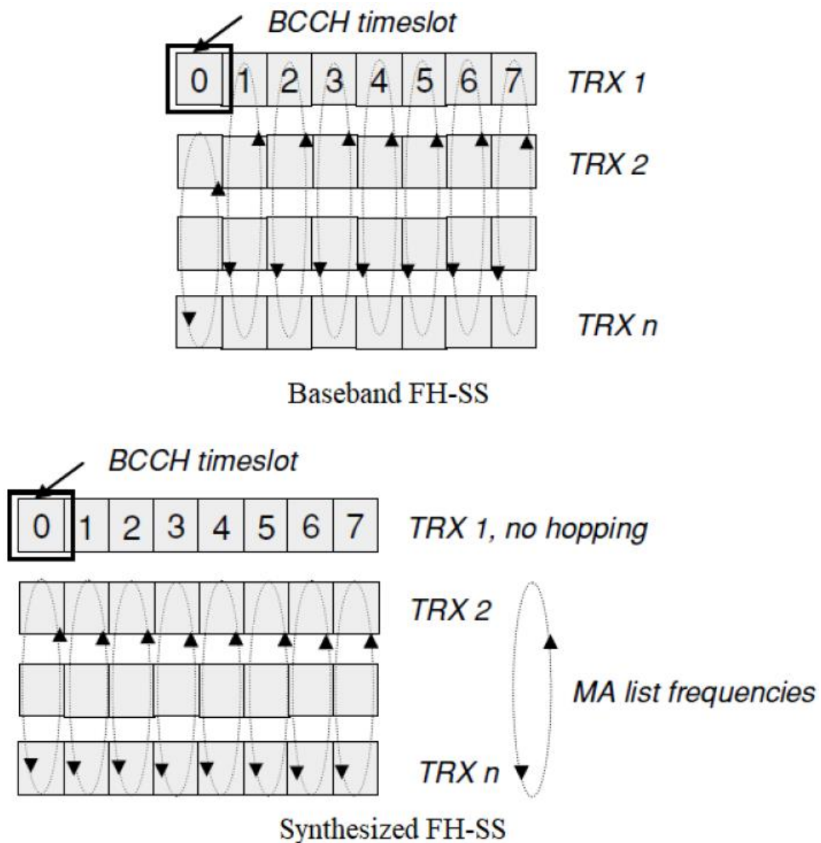
Figure 3 – Baseband FH-SS and synthesized FH-SS
