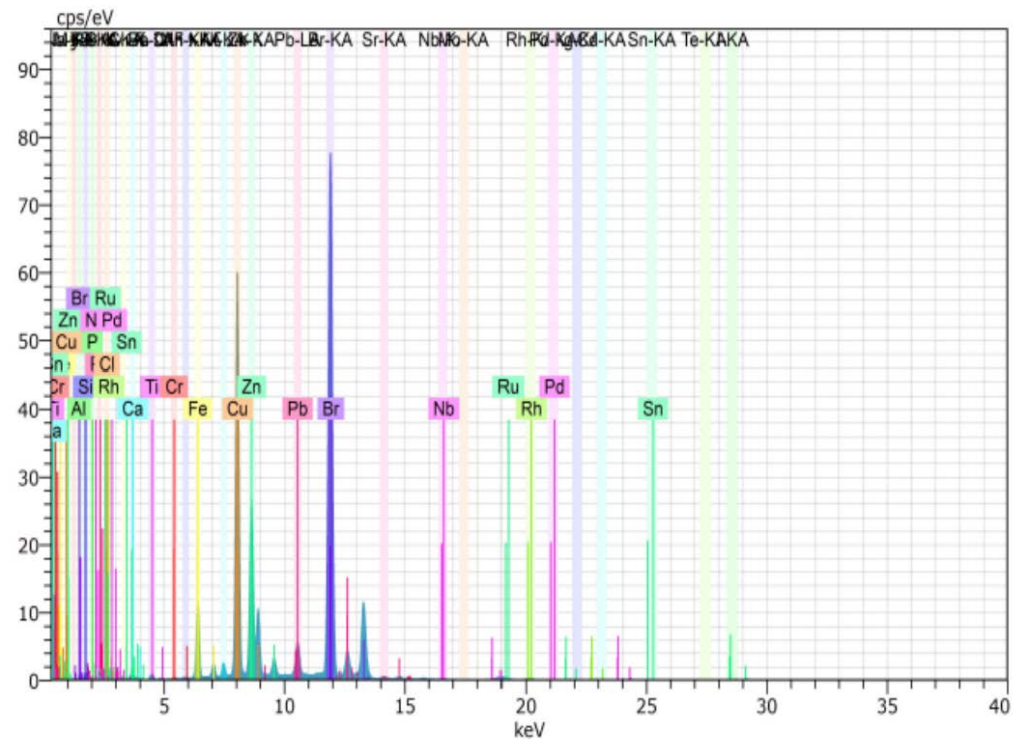
Figure 12. X-ray fluorescence spectrum of sample 10 for U=8 kV (non-conductor material)
