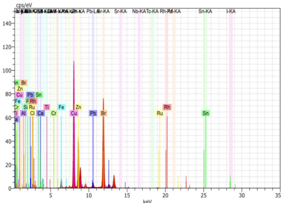
Figure 5. X-ray fluorescence spectrum of sample 3 for U=2kV (conductor material)
