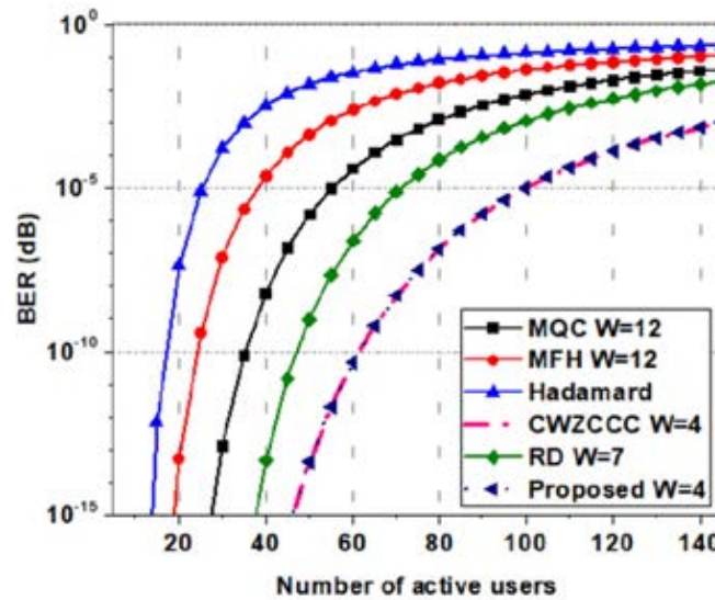
Figure 6. BER as a function of the number of users for different codes in the SACOCDMA system
