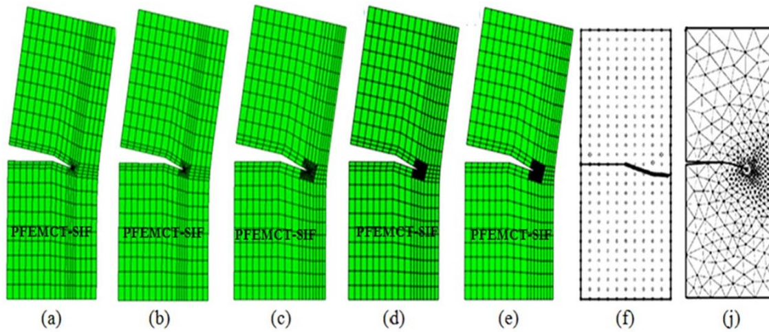
Figure 12. Crack propagation trajectory by the PFEMCT-SIF method: a) 3 contours, b) 5 contours, c) 10 contours, d) 15 contours, and e) 20 contours, (f) Phongthanapanich & Dechaumphai (2004) and (j) Rao & Rahman (2000)
