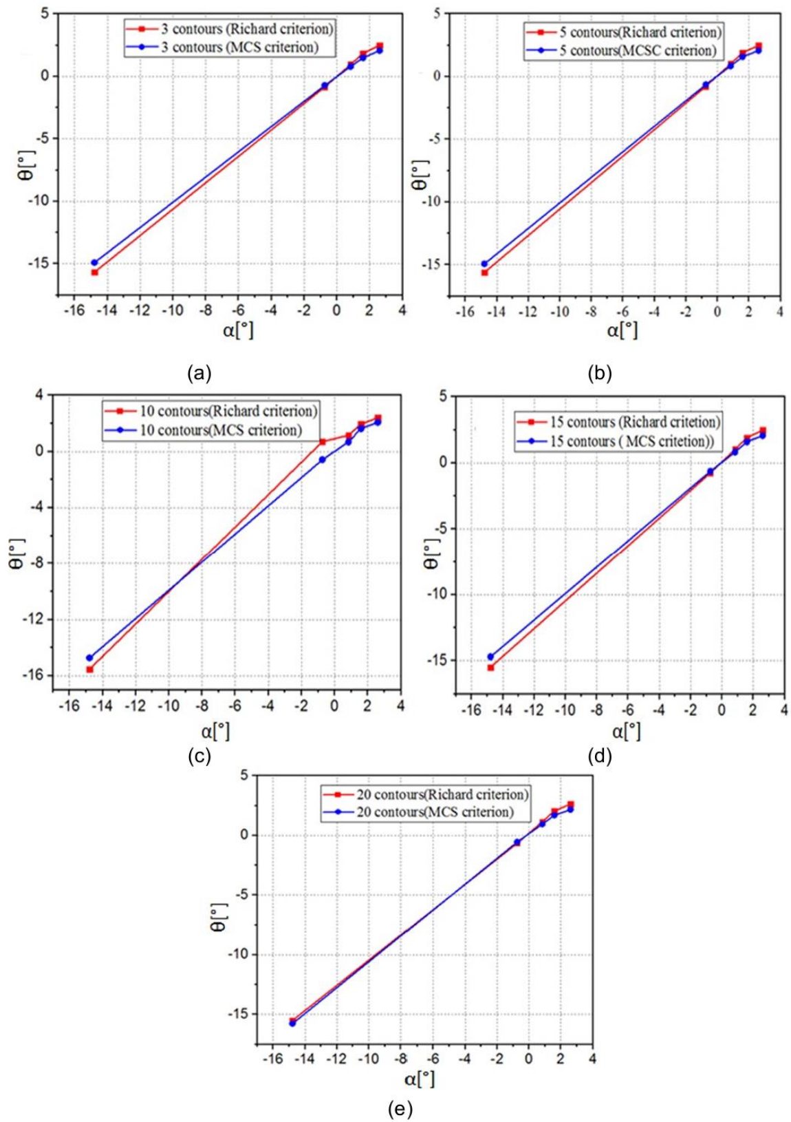
Figure 16. Comparison between the MCS and the Richard criterion by the PFEMCT-SIF; a) 3 contours, b) 5 contours, c) 10 contours, d) 15 contours, and e) 20 contours
