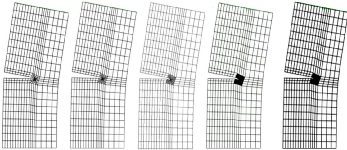
Figure 11. Crack propagation trajectory \alpha = -15.60^\circ : a) 3 contours, b) 5 contours, c) 10 contours, d) 15 contours, and e) 20 contours, by the PFEMCT-SIF method in the first propagation
