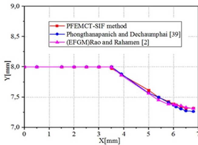
Figure 13. Comparison of the results between the three methods: Rao & Rahman (2000), Phongthanapanich & Dechaumphai (2004), and the PFEMCT-SIF method
