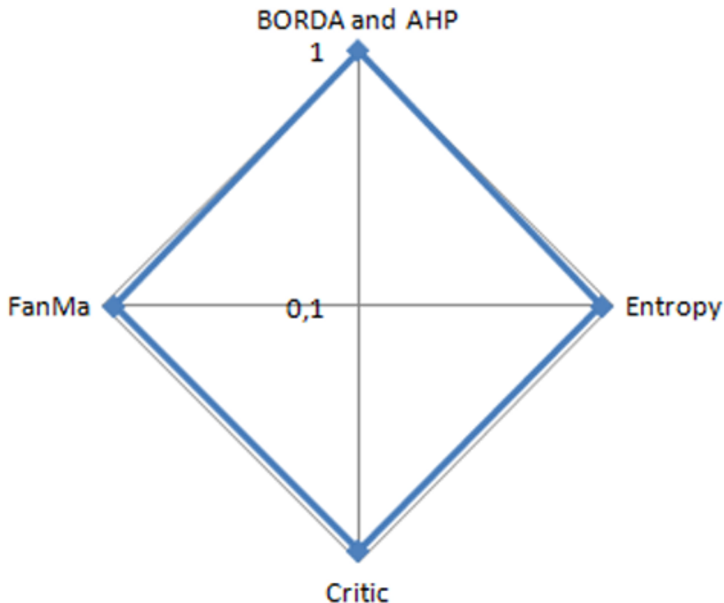
Figure 5. Spearman's rank correlation coefficient of the alternatives
