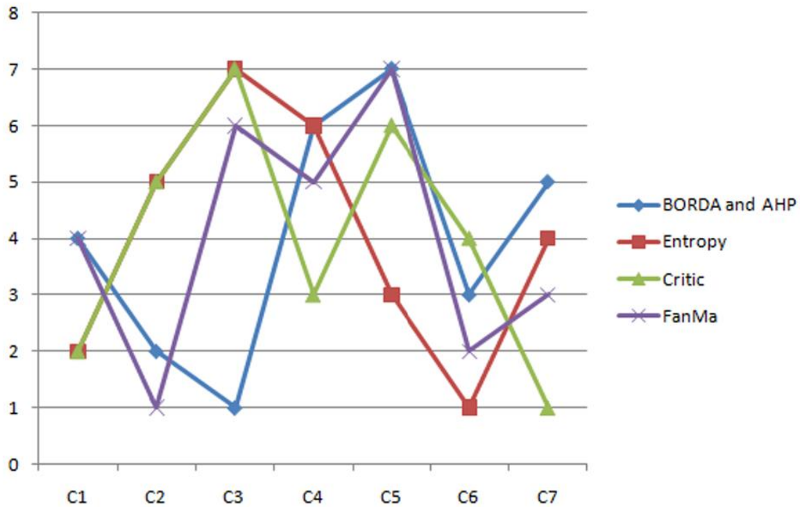
Figure 3. Graphical ranking of the criteria
