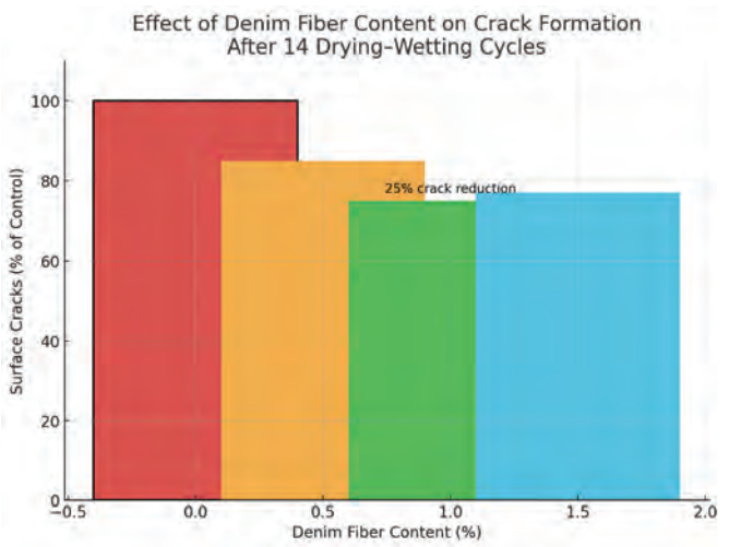
Figure 5: Diagram of denim fiber content affects surface crack formation after 14 drying-wetting cycles
