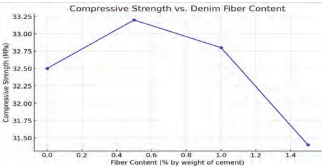
Figure 3: Compressive strength of concrete with varying denim fiber content at 7, 14, and 28 days.
