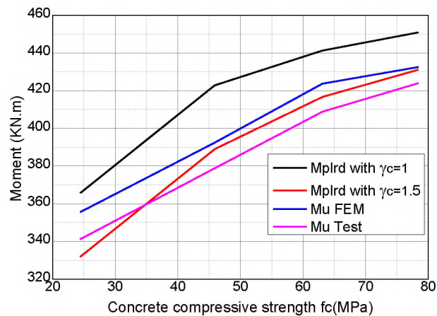
Figure 6 – Moment variation as a function of the concrete compressive strength
