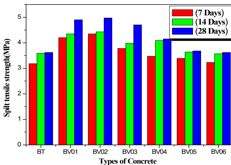
Figure 7 – Tensile strength of the concrete used
