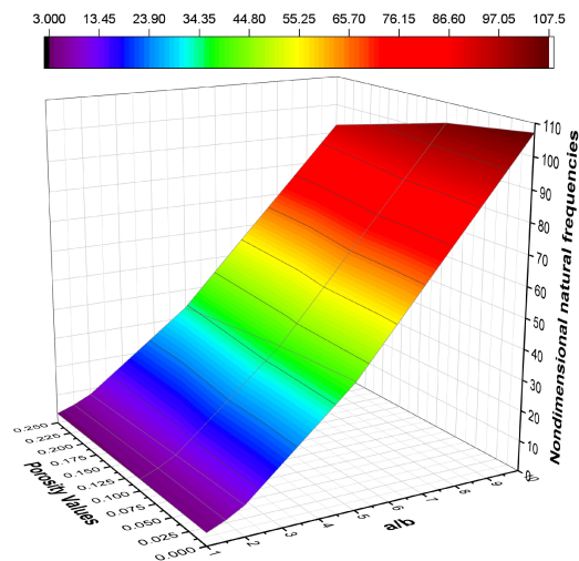
Figure 4 – 3D visualization of the effect of a/b and \alpha on the natural frequency \bar{\omega} for Al/Al_2O_3 plates ( p = 2 )
