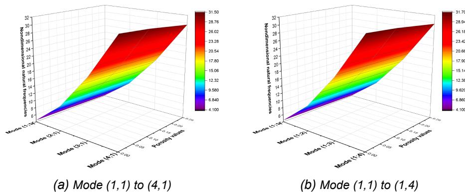
Figure 6 – Effect of mode shapes and \alpha on \bar{\omega} ( Al/Al_2O_3 plates)
