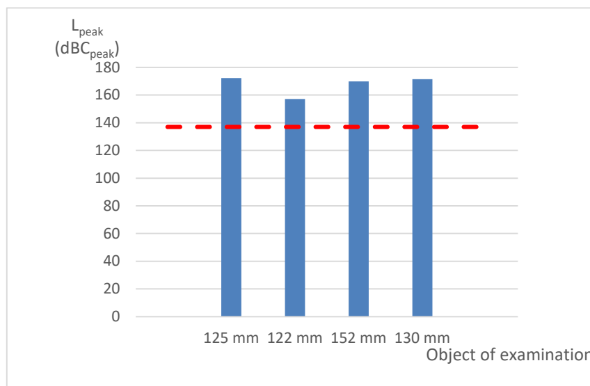
Diagram 5 - Summary of the peak noise level for all cannons in relation to the limit value
