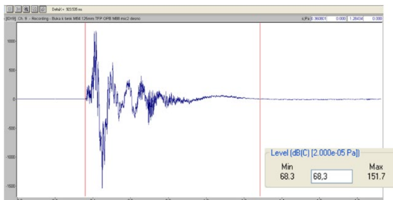
Diagram 2 - Noise curve produced by the 125 mm cannon at the commander's place
