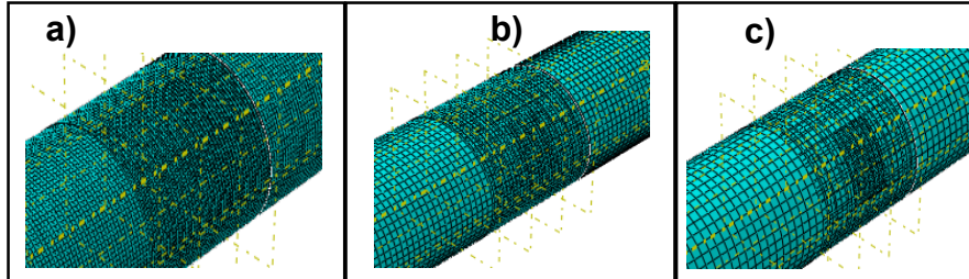
Figure 4 – Detailed mesh used for a numerical model of the defective pipe with composite repair: a) refined mesh, b) medium mesh, and c) non-refined mesh.
