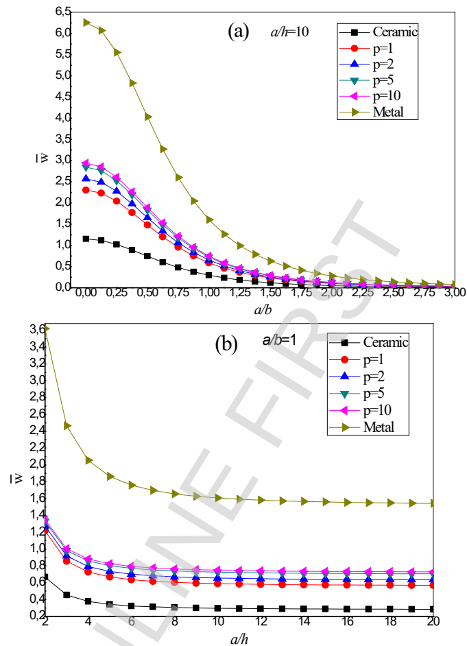
Figure 3 – \bar{w} vs ratios: (a) - a/b , (b) - a/h , of an S-FGM plate
