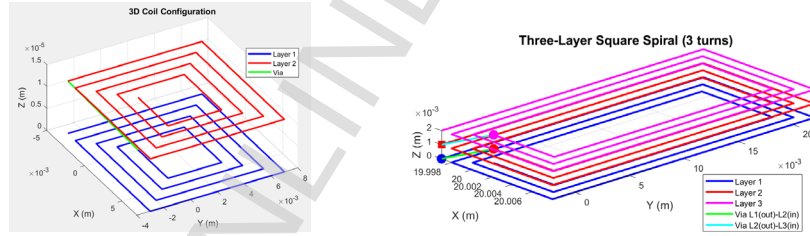
(a) 2-layer rectangular planar coil (b) 3-layer rectangular planar coil Figure 3 –3D representation of a 2-layer and 3-layer rectangular planar coil with spiral segments and via connections
