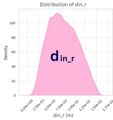
(e) Destitution of d_{in\_r}
