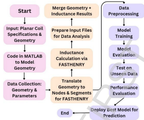
Figure 1 – Methodology flowchart for designing and predicting inductance of multilayer rectangular planar coils
