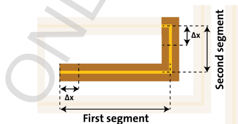
Figure 4 – Initial segments and design steps in the spiral creation
