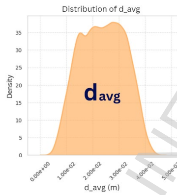
(g) Destitution of d_{avg}
