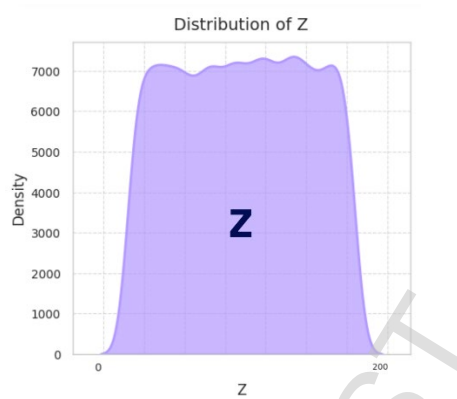
(k) Destitution of z
