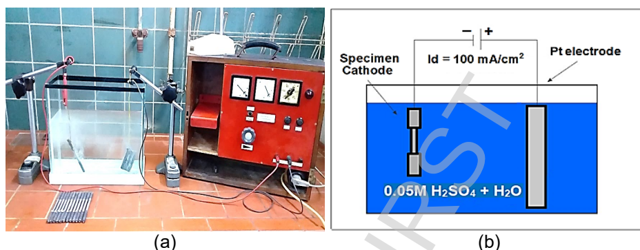
Figure 4 – (a) Hydrogen-loaded specimens in 0.05M ( \text{H}_2\text{SO}_4 ) ( \text{pH}=1.32 ) and (b) schematic of the experimental cathodic hydrogen charging (Depover et al., 2014)
