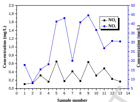
Figure 12 – Curve of the nitrite and nitrate ions content monitoring in the unhairing wastewater from the tannery, the Batna Unit
