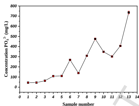
Figure 10 – Curve of the phosphate ion content monitoring in the unhairing wastewater from the tannery, the Batna Unit
