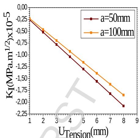
Figure 13 - Effect of Imposed Displacement U on Mode I Propagation of a Crack ( U > 0 , Tension)
