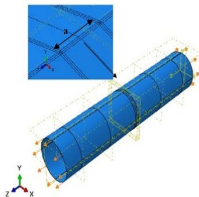
Figure 12 - Boundary conditions for a pipeline with a longitudinal crack subjected to tensile forces ( U > 0 )
