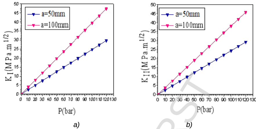
Figure 7- Effect of Internal Pressure on the Mode I and Mode II Behaviour of a Crack Oriented at 45^\circ
