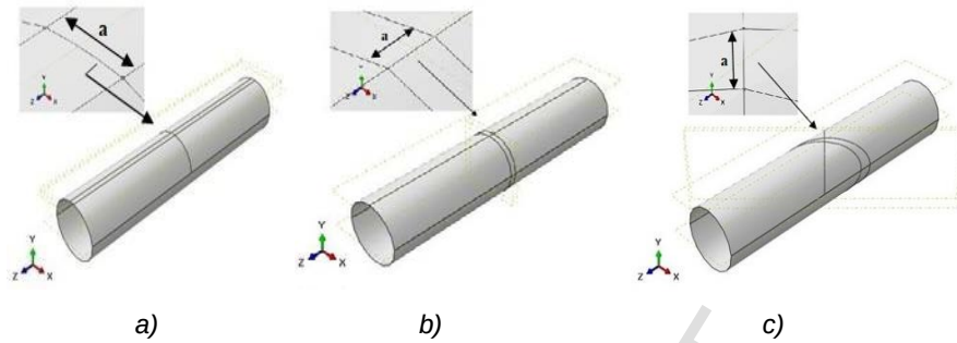
Figure 1 - Pipeline containing a crack: (a) circumferential, (b) longitudinal, (c) mixed (45° orientation)
