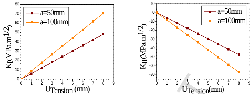
Figure 18 - Effect of Imposed Displacement U on the Propagation Kinetics in Modes I and II of a Crack Oriented at 45^\circ ( U > 0 , Tension)
