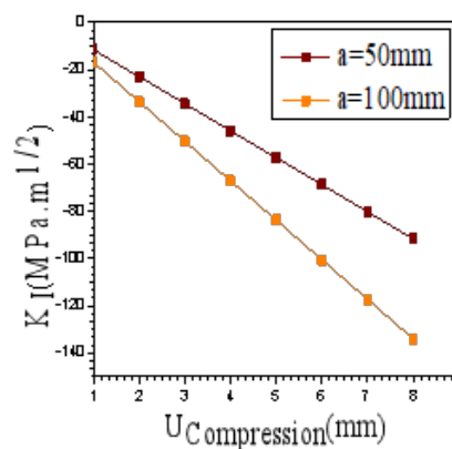
Figure 11 - Effect of Imposed Displacement U on Mode I Propagation of a Crack ( U < 0 , Compression)
