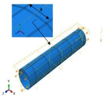
Figure 8 - Boundary conditions for a pipeline with a circumferential crack subjected to tensile forces ( U > 0 )
