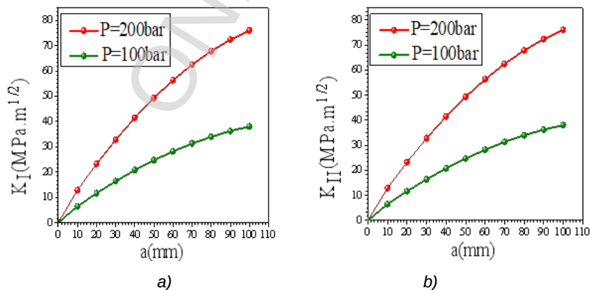
Figure 6 - Behaviour of a Crack of Size "a" Oriented at 45° in Modes I and II
