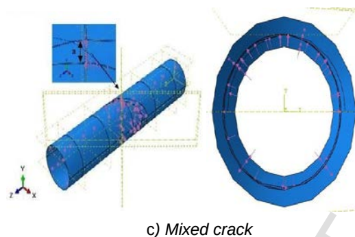
Figure 2 - Boundary conditions applied to the cracked pipeline under internal pressure
