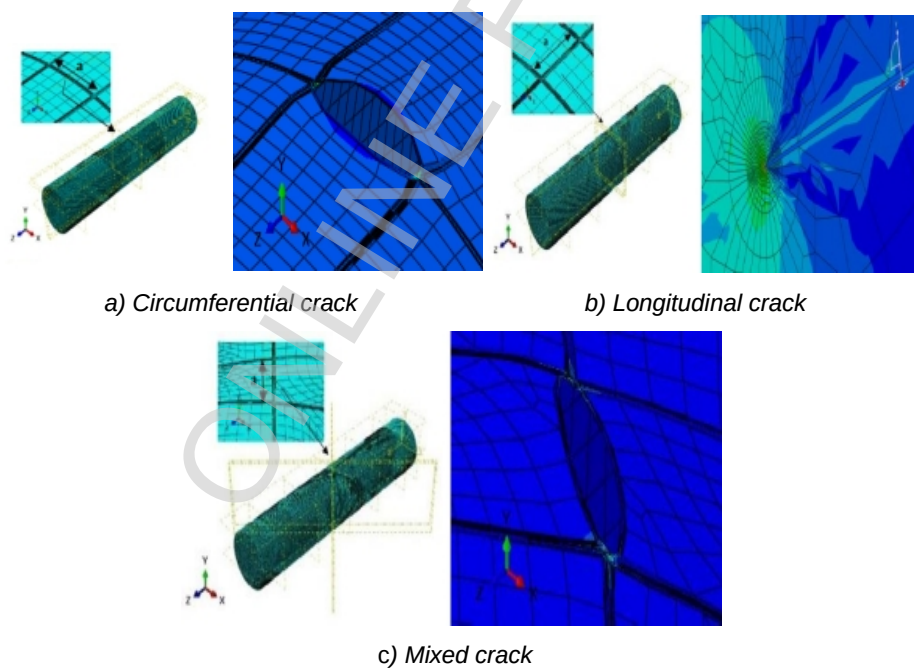
Figure 3 - Mesh of the analysed structure
