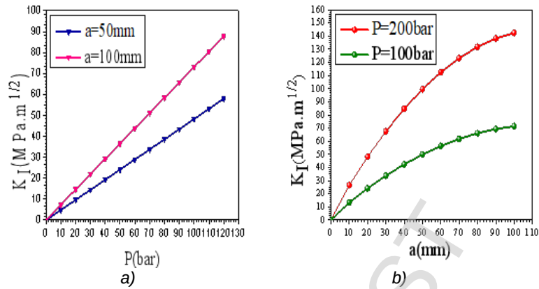
Figure 5 - Effect of Pressure and Longitudinal Crack Size on its Propagation Kinetics in Mode I
