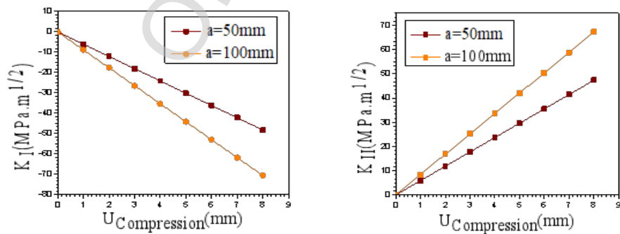
Figure 19 - Effect of Imposed Displacement U on the Propagation Kinetics in Modes I and II of a Crack Oriented at 45^\circ ( U < 0 , compression)
