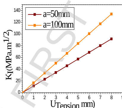
Figure 9 - Effect of Imposed Displacement U on Mode I Propagation of a Crack ( U > 0 , Tension)
