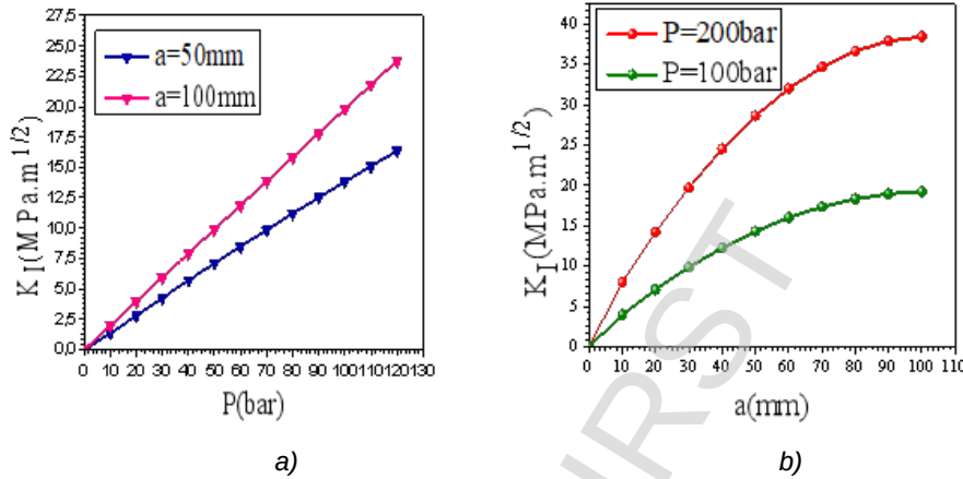
Figure 4 - Effect of Pressure and Circumferential Crack Size on its Propagation Kinetics in Mode I
