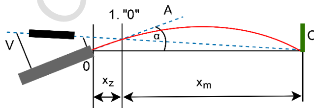
Figure 1 - Zeroing distance
