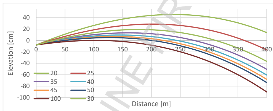
Figure 5 - Bullet flight path
