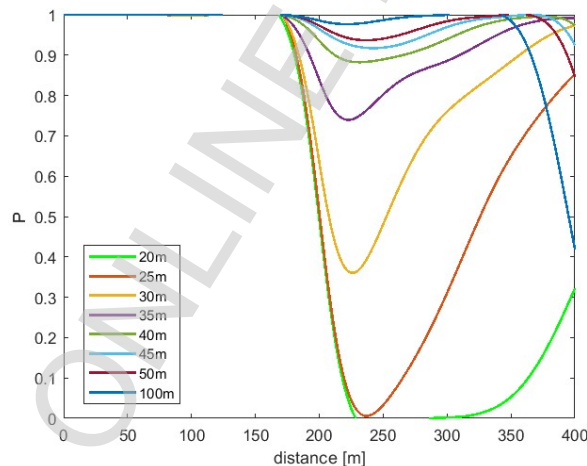
Figure 6 - Hit probability (prone, E-type) with aim point shift at 200 m
