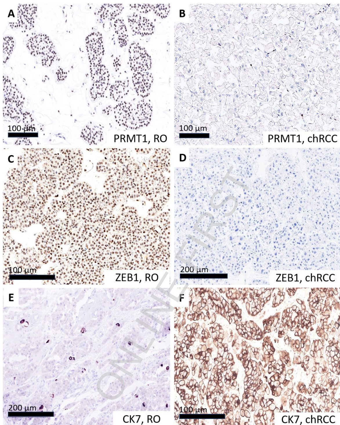
Figure 2. Representative microphotographs of PRMT1, ZEB1, and CK7 expression in RO and chRCC show: (A) high PRMT1 expression in the majority of RO and (B) its absence in most chRCC cases; (C) high nuclear ZEB1 expression in the majority of RO, whereas (D) all chRCC cases were negative for ZEB1; (E) CK7 expression was absent in the majority of RO, while (F) diffuse membranous CK7 staining was present in most chRCC cases: microscope magnification, 100 \times .
