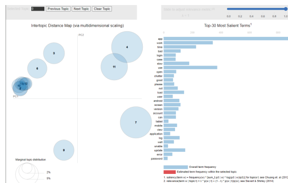
Figure 1: Visualization of topics in negative sentiment reviews using the pyLDAvis library
