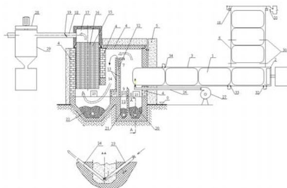
Sl. 1. Šema kotla za sagorevanje malih bala poljoprivredne biomase Fig. 1. Scheme of the small agricultural biomass bale combustion boiler
