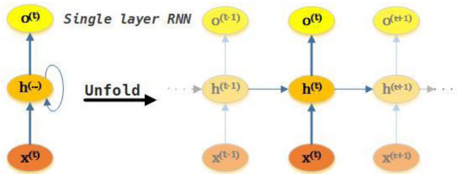
Figure 3. Unfolded RNN
