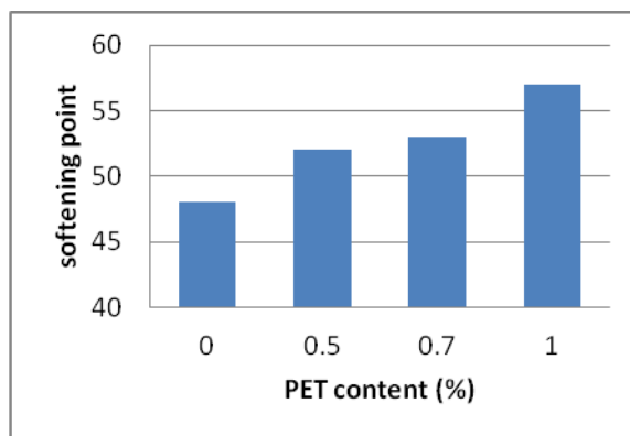
Figure 3. Softening point of modifier asphalt
