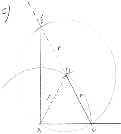
Figure 3. Abu'l Wafa's solution.
