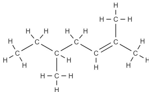
Figure 2. The Structural Formula of Alkene that had to be Identified in Item 5.
