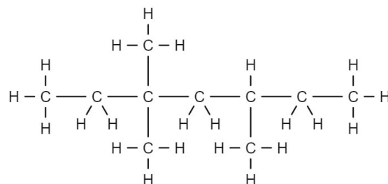
Figure 1. The Structural Formula of Alkane that had to be Identified in Item 1.
