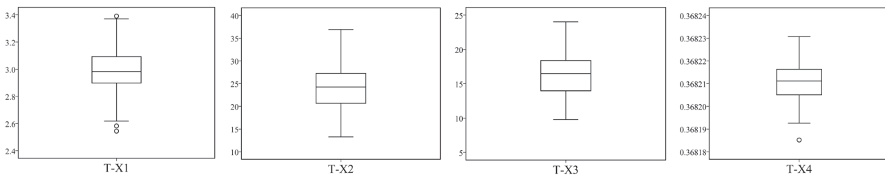
Figure 4: Box-plots of transformed variables
