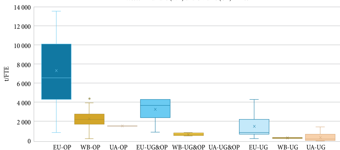
Figure 5: Lignite mines productivity comparisons in volume per full-time employee (FTE)
