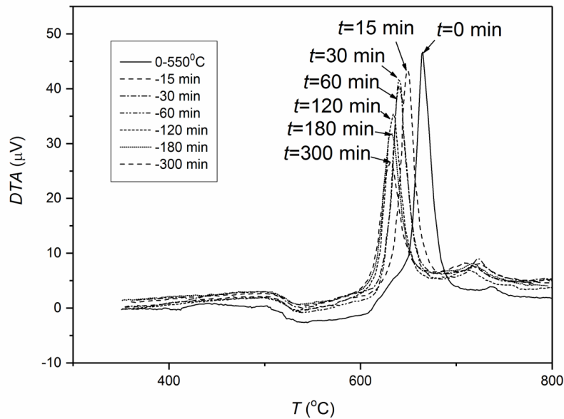
Figure 2 Differential thermal analysis curves of glass powders with particle sizes between 0.5 and 0.65 mm, subjected to annealing at 550 °C for different times.
