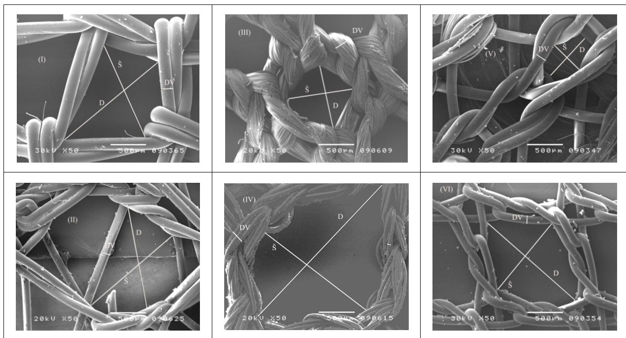
Figure 1. Scan electron microscope graft images (50/1) (I-HWPP, II-LWPP, III-MPP, IV-MPPG, V-CPP, VI-TPP, \checkmark -pore size, D-pore length, DV-filament thickness)
