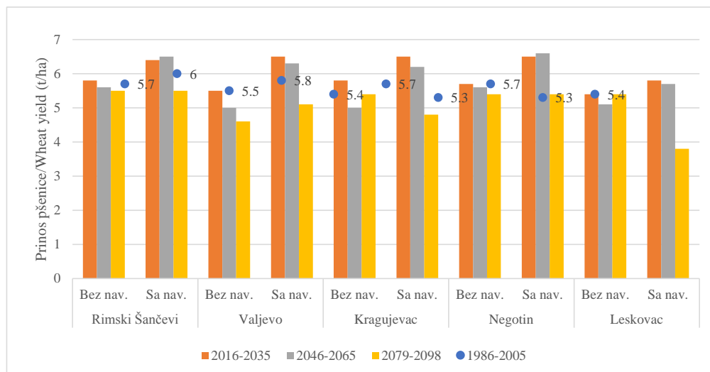
Grafik 5. Simulirani prinosi pšenice u uslovima sa i bez navodnjavanja ( t\ ha^{-1} ) Figure 5. Simulated yield of rainfed and irrigated wheat ( t\ ha^{-1} )
