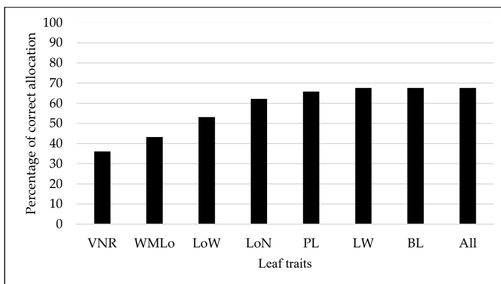
Figure 6. Percentage of correct classification for models generated based on stepwise discriminant analysis.
