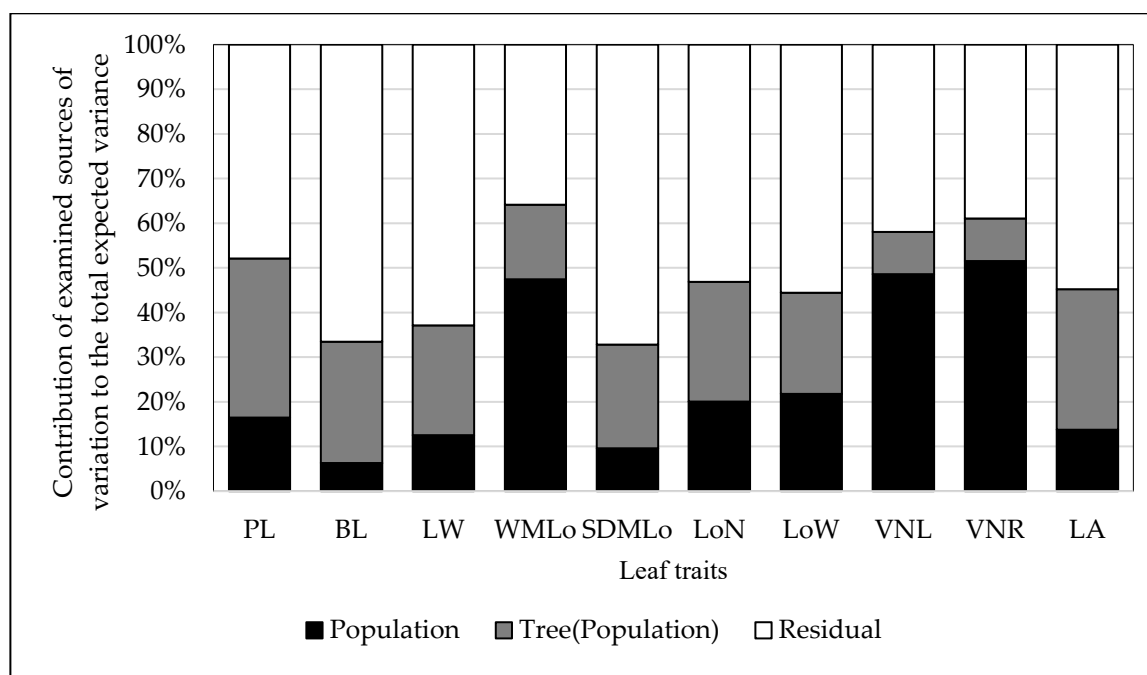
Figure 3. Contribution of the examined sources of variation to the total expected variance for the measured parameters of the studied Quercus robur L. populations.
