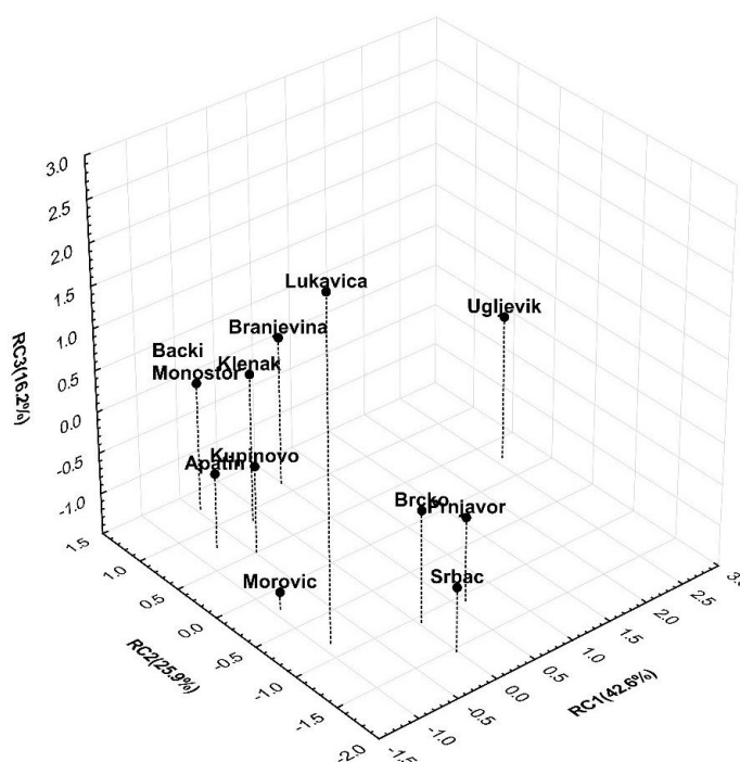
Figure 4. Ordination of the studied Quercus robur L. populations based on the first three principal components following Varimax rotation.
