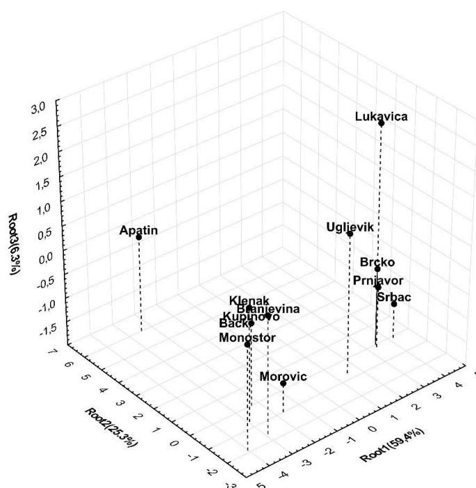
Figure 5. Relationship among the studied Quercus robur L. populations based on the first three canonical variables.
