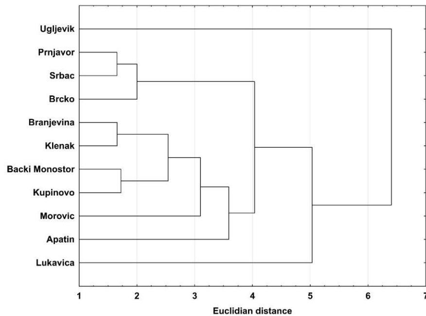
Figure 7. Dendrogram of the cluster analysis of the studied Quercus robur L. populations, aggregated using the UPGMA method based on standardized measured parameters.
