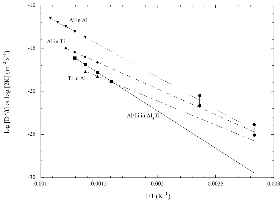
Figure 7. Arrhenius plots of (●) \log (D^2/t) from this study where D is the observed domain size and t is a typical range of deposition times (2 to 30 h); and \log (2K) where K is a literature value of the diffusion coefficient of (▲) Ti in Al [47], (◆) Al in Ti [48], (▼) Al in Al [49], and (■) interdiffusion coefficient of Ti and Al in Al 3 Ti [50]. The lines are an extrapolation of the literature data to the deposition temperature range examined in this study.
