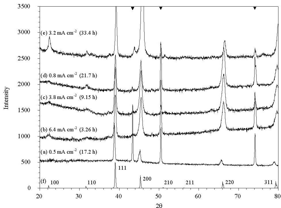
Figure 3. X-ray diffraction patterns (Cu K\alpha ) of Al-Ti alloys electrodeposited from (a) 2:1 AlCl_3 -EtMeImCl electrolyte containing 170 \text{ mmol L}^{-1} \text{ Ti}^{2+} at 80^\circ \text{C} and (b-e) 2:1 AlCl_3 -NaCl electrolyte containing 150 \text{ mmol L}^{-1} \text{ Ti}^{2+} at 150^\circ \text{C} . The composition, current density and total charge for the deposits are (a) 18.4 % Ti, 0.5 \text{ mA cm}^{-2} , 31.0 \text{ C cm}^{-2} ; (b) 25.1 % Ti, 6.4 \text{ mA cm}^{-2} , 75.3 \text{ C cm}^{-2} ; (c) 25.8 % Ti, 3.8 \text{ mA cm}^{-2} , 125.3 \text{ C cm}^{-2} ; (d) 26.3 % Ti, 0.8 \text{ mA cm}^{-2} , 62.5 \text{ C cm}^{-2} ; (e) 23.5 % Ti, 3.2 \text{ mA cm}^{-2} , 385.0 \text{ C cm}^{-2} ; (f) calculated diffraction pattern for fully ordered ( L1_2 ) Al_3\text{Ti} [23]. Copper reflections from substrate denoted by ( \blacktriangledown ) at the top of the figure [51].
