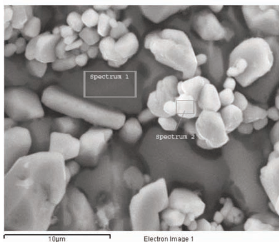
Figure 7. SEM micrograph of the leach residue: T = 80^{\circ}\text{C} , t = 240 \text{ min} , stirring speed = 300 rpm, [\text{H}_2\text{SO}_4] = 1.5 \text{ M} , [\text{NaNO}_3] = 0.6 \text{ M} , phase ratio 20 g/1.2dm 3
