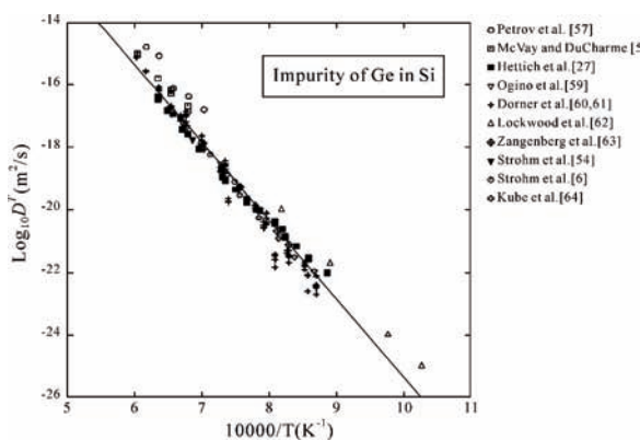
Figure 4. Impurity diffusivities of Ge in Si. The symbols are the reported diffusivities in the literature [6, 27, 54, 57-64], while the solid line is calculated according to the present atomic mobility parameters.
