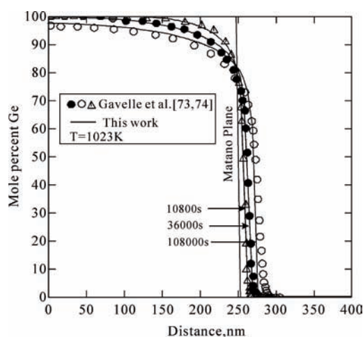
Figure 16. Model-predicted concentration profiles of Ge/Si thin layer diffusion couples annealed at 1023 K in comparison with the experimental data from Gavelle et al. [73, 74].
