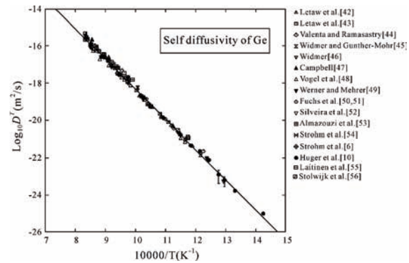
Figure 3. Self diffusivities of Ge. The symbols are the reported diffusivities in the literature, while the solid line is calculated according to the present atomic mobility parameters [6, 10, 42-56].
