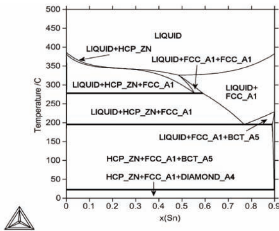
Figure 8. Isopleth of the Al-Sn-Zn system for 10 at% Sn (FCC_A1=(Al), HCP_ZN=(Zn), BCT_A5=( \beta Sn), DIAMOND_A4=( \alpha Sn))
