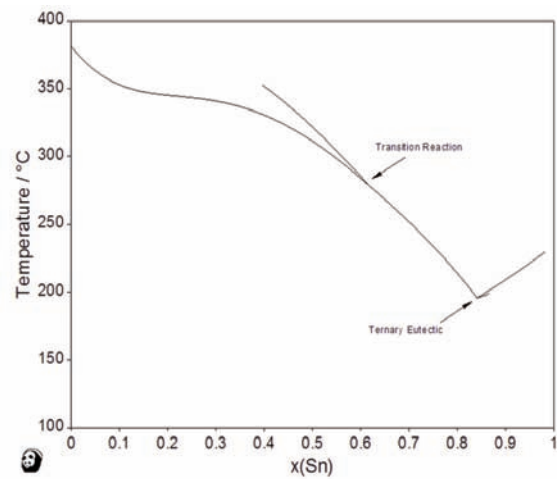
Figure 10. Liquidus projection on on to the T - x plane for the Al-Sn-Zn syste
