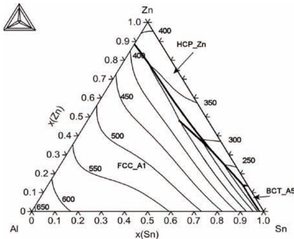
Figure 9. Liquidus projection of the Al-Sn-Zn system (from [25], (FCC_A1=(Al), HCP_ZN=(Zn), BCT_A5=( \beta Sn)).
