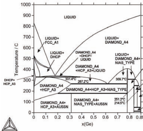
Figure 7. Isopleth of the Au-Ge-Sn system for 11 at% Sn (NIAS_TYPE=AuSn/ \delta , DHCP= Au_{10}Sn/\beta , FCC_A1=(Au), BCT_A5=(Sn), HCP_A3= \zeta , PTSN4_TYPE=AuSn _4 )
