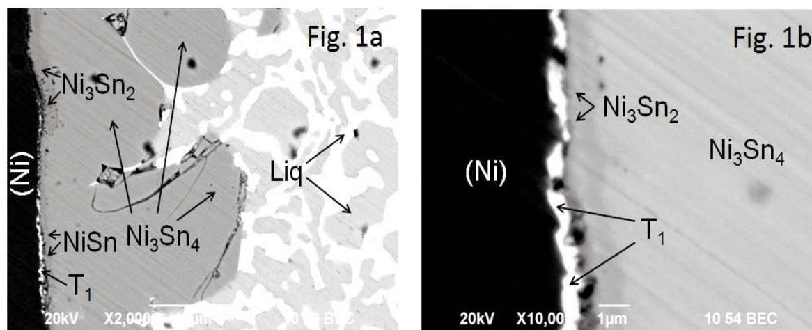
Figure 1. a, b. Micrographs of sample No. 11 (annealed at 370^\circ\text{C} ) in back scattered electrons. a) The main diffusion layer is of \text{Ni}_3\text{Sn}_4 phase; the (former) liquid phase (Liq) consists of light (Bi-rich) and darker Sn-rich (areas); ternary phase ( T_1 ) is observed as white layer between (Ni) and \text{Ni}_3\text{Sn}_2 -layer; NiSn layer is situated between \text{Ni}_3\text{Sn}_2 and \text{Ni}_3\text{Sn}_4 layers. b) Magnified region of sample No. 11. The white layer belonging to the T_1 phase is well seen.
