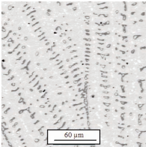
Figure 6. BSE-SEM image of nominal \text{Pt}_{18}:\text{Al}_2:\text{Cr}_{80} (Alloy 16) after annealing at 1000^\circ\text{C} : (Cr) dark; \sim\text{Cr}_3\text{Pt} medium; \tau_1 white.
