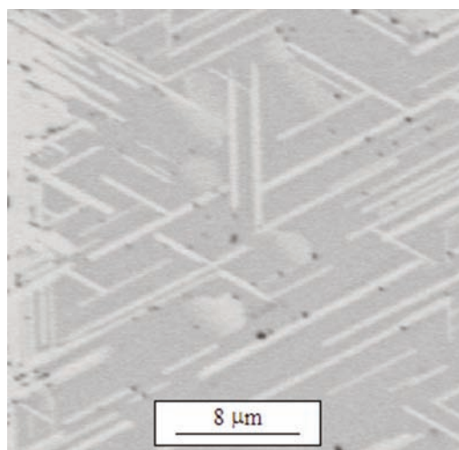
Figure 8. BSE-SEM image of nominal \text{Pt}_{34}:\text{Al}_{49}:\text{Cr}_{17} (Alloy 23) after annealing at 1000°C: (Cr) black; \sim\text{Pt}_2\text{Al}_3 + \sim\text{PtAl}_2 medium; \sim\text{PtAl} white.
