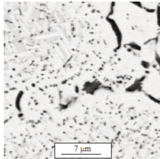
Figure 7. (a). BSE-SEM image of nominal \text{Pt}_{30}:\text{Al}_{50}:\text{Cr}_{20} (Alloy 21) after annealing at 1000^\circ\text{C} : (Cr) dark; \sim\text{PtAl}_2 medium; \sim\text{Pt}_2\text{Al}_3 white; (b) Higher magnification of interdendritic region.
