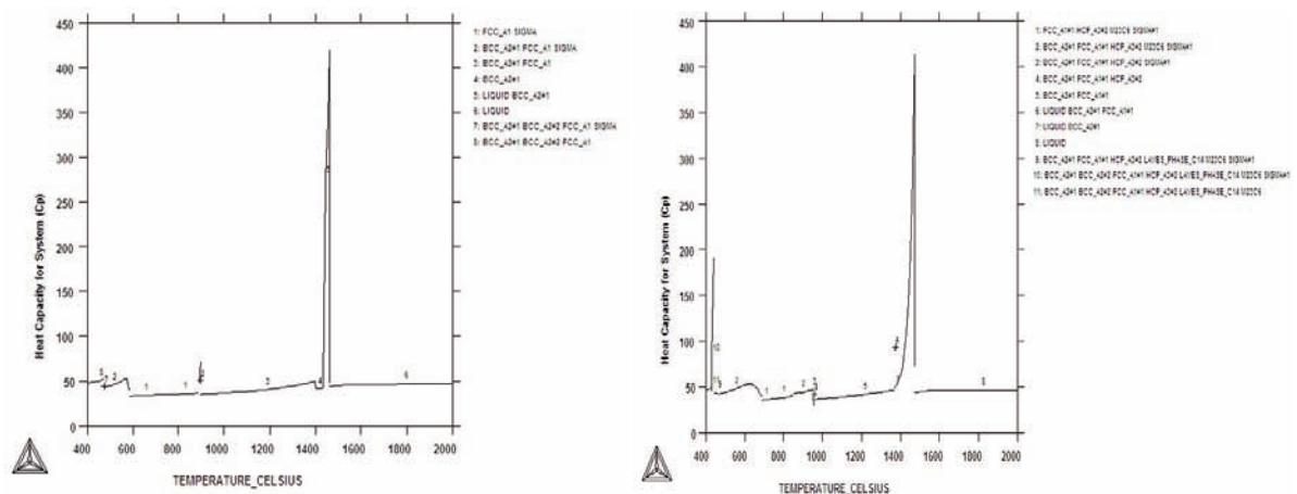
Figure 5. Specific heat (Lever) for duplex-SAF 2205 in Jmol -1 K -1 ; gas suspended: (a) calculation is based on nickel and chromium equivalent and (b) calculation using complete chemical composition.
