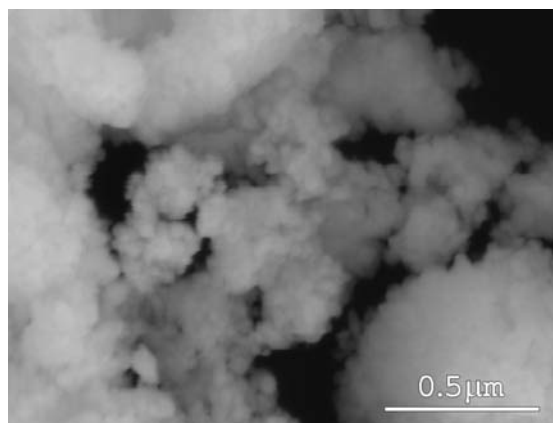
Figure 3. Structure of the Sn-5.91wt%Ag nanoalloy synthesized at -20^\circ\text{C} (SEM, av. particle size 40 nm and agglomerate \approx 1\mu\text{m} (right bottom)).
