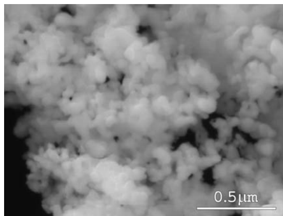
Figure 2. Structure of the Sn-7.84wt%Ag nanopowder synthesized at -10^\circ\text{C} (SEM, av. particle size 60 nm).
