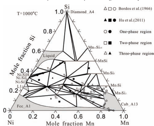
Figure 3. Calculated isothermal section at 1000 °C of the Mn-Ni-Si system along with the experimental data from Hu et al. [1] and Bordos et al. [12].
