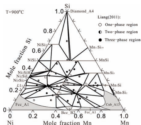
Figure 2. Calculated isothermal section at 900 °C of the Mn-Ni-Si system along with the experimental data from Liang [7].
