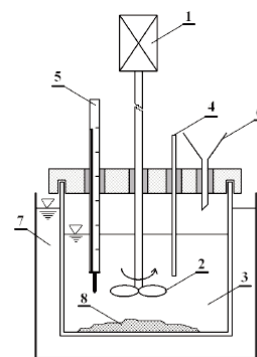
Figure 6. The scheme of the leaching apparatus [26]: 1 – stirrer engine; 2 – propeller; 3 – leaching pulp; 4 – sampler; 5 – thermometer; 6 – feeder; 7 – water thermostat; 8 – sample
