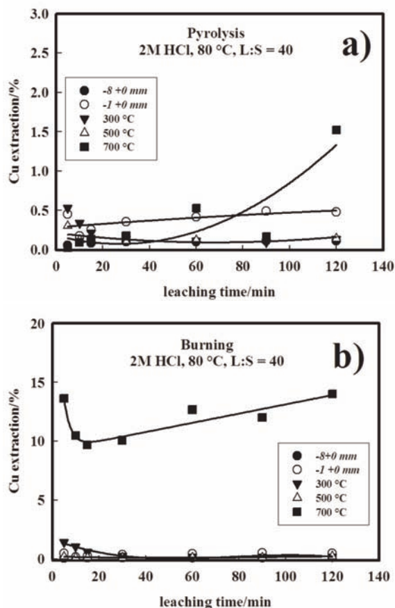
Figure 11. a, b Copper leaching curves a) pyrolyzed samples; b) burned samples
