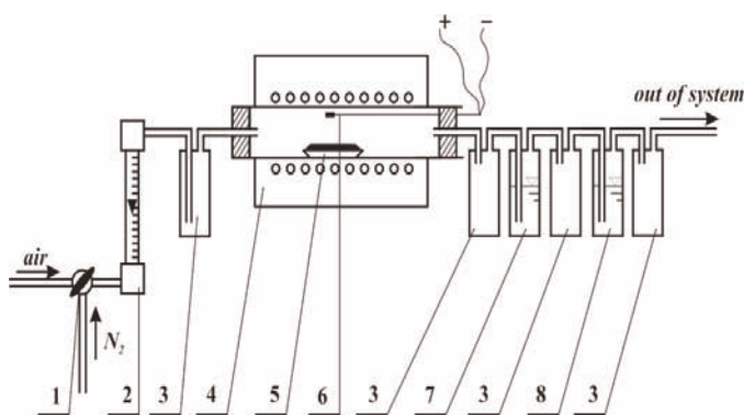
Figure 5. The scheme of the apparatus for thermal treatment: 1 – tap, 2 – volumeter, 3 – empty bubbler, 4 – laboratory furnace, 5 – ceramic sample boat, 6 – thermocouple, 7 – NaOH solution, 8 – H_2SO_4 solution
