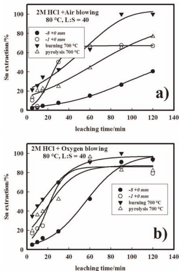
Figure 12. a, b Tin leaching curves in 2M HCl with blowing air and oxygen
