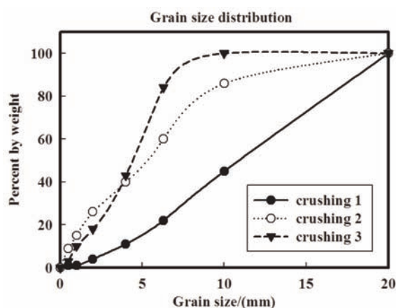
Figure 4. Cumulative curves of material after crushing
