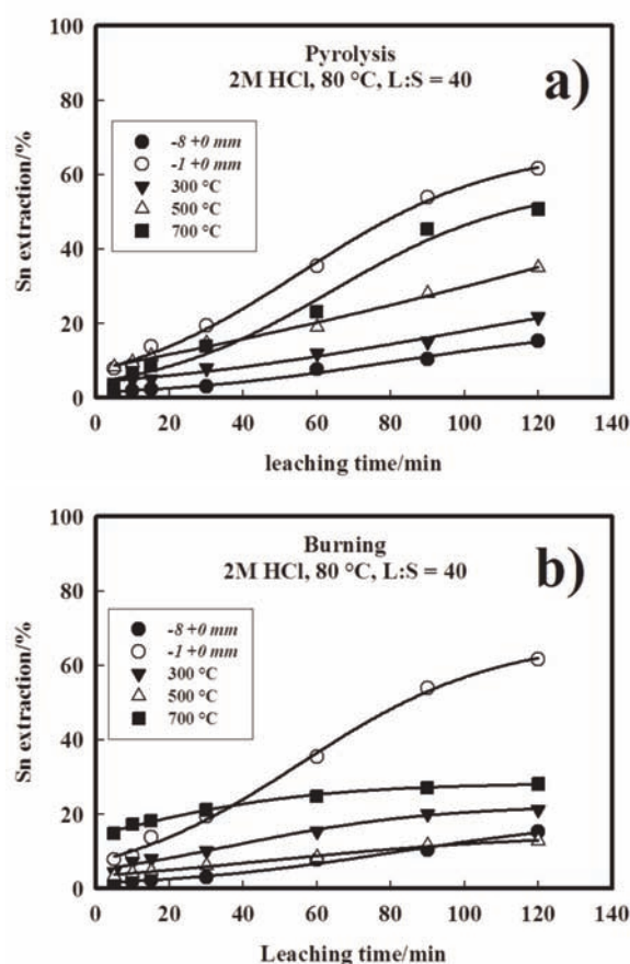
Figure 10. a, b Tin leaching curves a) pyrolyzed samples; b) burned samples
