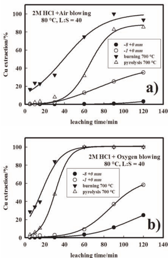
Figure 13. a, b Copper leaching curves in 2M HCl with blowing air and oxygen
