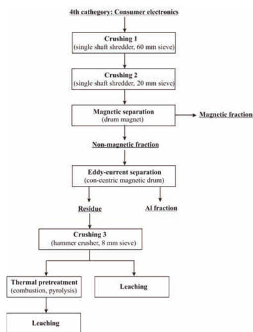
Figure 2. Overall scheme of realized experiments
