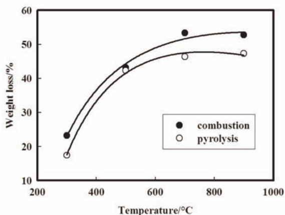
Figure 7. Temperature dependence of weight losses after burning and pyrolysis
