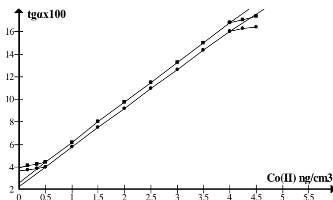
Figure 5. Effect of Co(II) concentration on the reaction rate. Experimental conditions: 2 × 10 -4 mol/dm 3 of KMnO 4 , 1.5 × 10 -4 mol/dm 3 of 4-OHcoum., pH=3.8. (•)-temperature 25 ± 0.1 °C, (▪)-temperature 30 ± 0.1 °C
