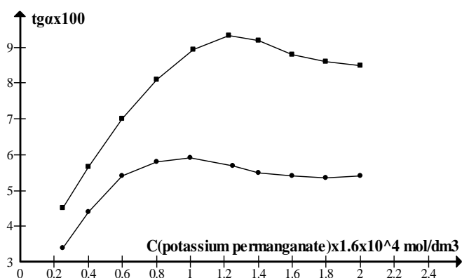
Figure 4. Effect of KMnO 4 concentration on determination of Co(II). Experimental conditions: 1.5 × 10 -4 mol/dm 3 of 4-OHcoum., 5 ng/cm 3 of Co(II), pH=3.8. (▪)-catalytic reaction, (•)-non-catalytic reaction.
