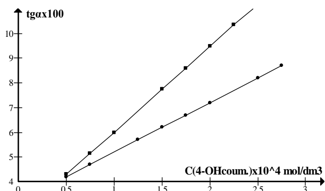
Figure 3. Effect of 4-OHcoum. concentration on determination of Co(II). Experimental conditions: 2 × 10 -4 mol/dm 3 of KMnO 4 , 5 ng/cm 3 of Co(II), pH=3.8. (▪)-catalytic reaction, (•)-non-catalytic reaction.
