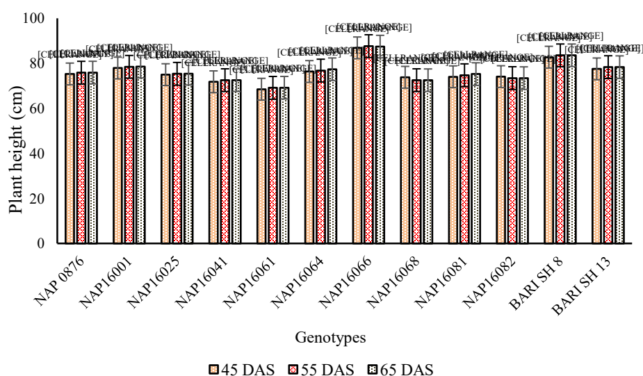
Figure 2. Plant height (cm) of 12 genotypes of Brassica napus recorded at different dates after sowing.
