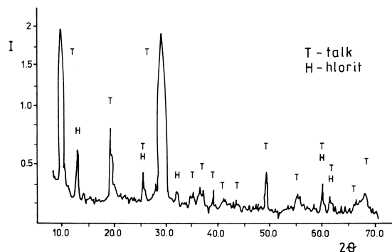
Figure 5. Roentgenogram of lining T suspension.
