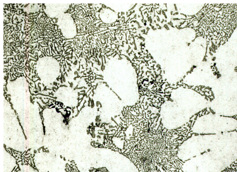
Figure 9. Microstructure of casting series C
