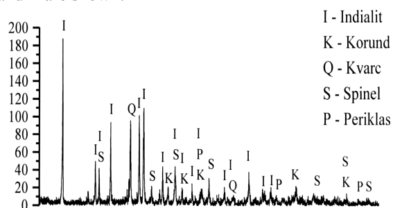
Figure 4. Roentgenogram of lining C suspension.
