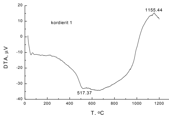
Figure 6. DTA curve of sample C.
