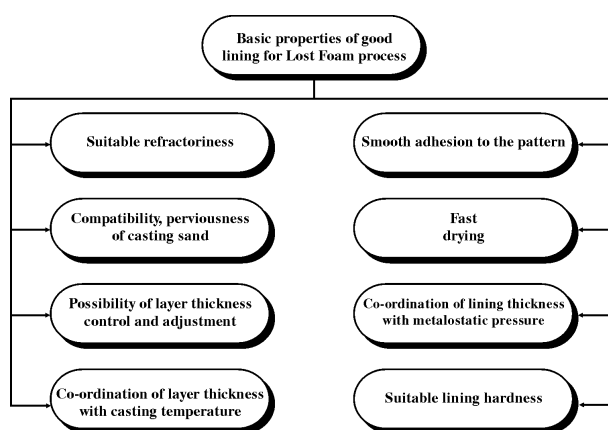
Figure 1. Basic ceramic lining properties in the Lost Foam process.
