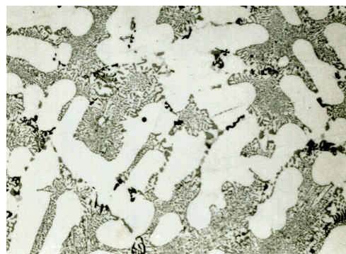
Figure 10. Microstructure of casting series T
