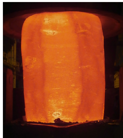
Figure 8. Approbation a new process forging of the workpiece with weight 57.7 ton (upsetting process)
